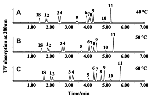
Figure 3. SFC chromatograms of (A) column temperature 40°C, (B) column temperature 50°C, and (C) column temperature 60°C, all at backpressure 135 bar. For peak labels, see Table 1. Chromatographic conditions: methanol (20 mM citric acid) 1.5%, 0–2 min; 1.5–9%, 2–5 min; 9%, 5–6 min; 9–1.5%, 6–7 min. Flow rate 1.0 mL/min. Detection at 280 nm.
