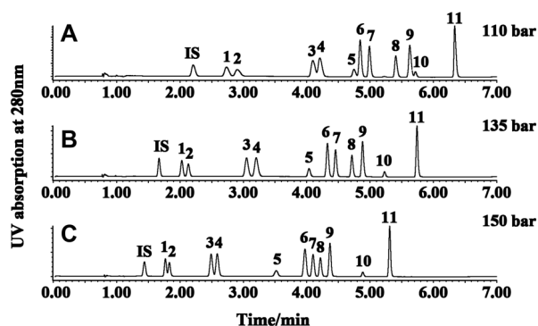
Figure 4. SFC chromatograms of (A) backpressure 110 bar, (B) backpressure 135 bar, (C) backpressure 150 bar, all at column temperature 60°C. For peak labels, see Table 1. Chromatographic conditions: methanol (20 mM citric acid) 1.5%, 0–2 min; 1.5–9%, 2–5 min; 9%, 5–6 min; 9–1.5%, 6–7 min. Flow rate 1.0 mL/min. Detection at 280 nm.
